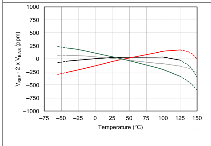
Figure 11. V_{REF} - 2 \times V_{BIAS} Tracking vs Temperature
