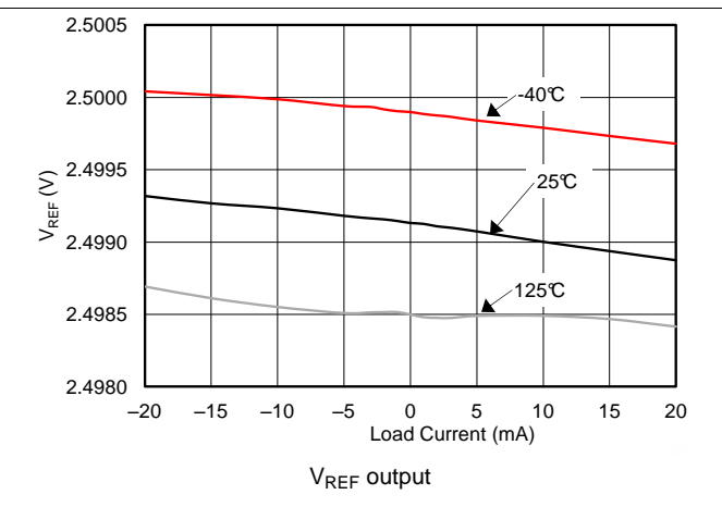
Figure 12. Output Voltage Change vs Load Current ( V_{REF} )
