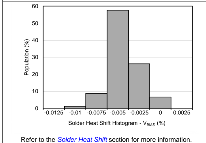
Figure 9. Solder Heat Shift Distribution ( V_{BIAS} )
