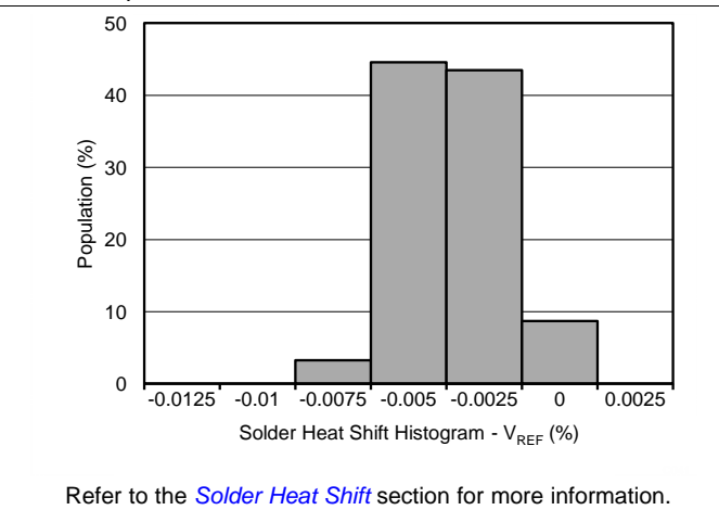
Figure 8. Solder Heat Shift Distribution ( V_{REF} )
