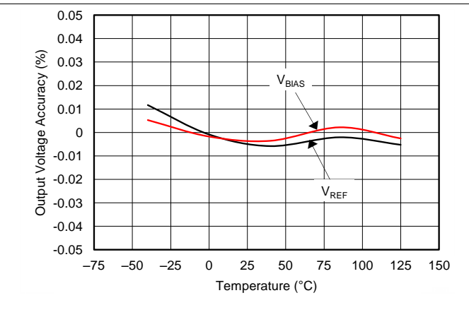
Figure 10. Output Voltage Accuracy ( V_{REF} ) vs Temperature
