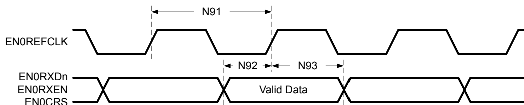
Figure 27-43. RMII Receive Timing
