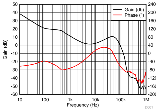
Figure 57. Gain and Phase Plot
