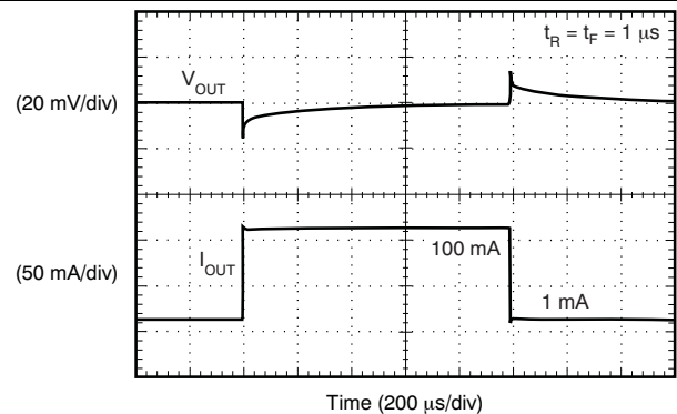
Figure 16. Load Transient 0
