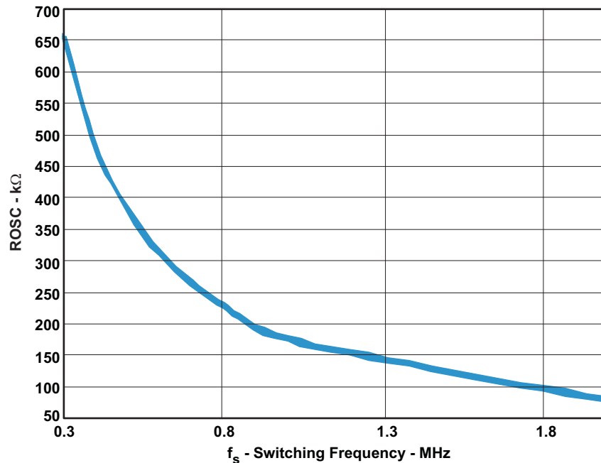
Figure 38. ROSC vs Switching Frequency
