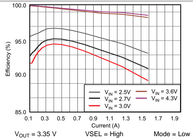
Figure 32. TPS61281A Efficiency vs Output Current
