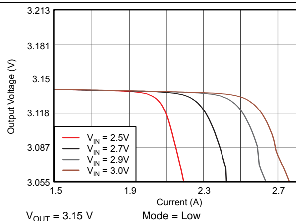
Figure 34. TPS61281A DC Output Voltage vs Output Current
