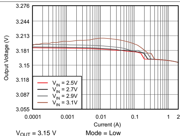
Figure 33. TPS61281A DC Output Voltage vs Output Current
