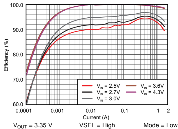
Figure 31. TPS61281A Efficiency vs Output Current
