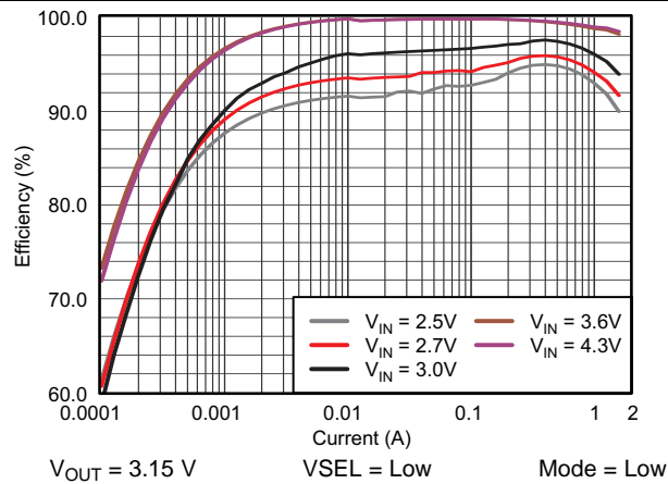
Figure 29. TPS61281A Efficiency vs Output Current
