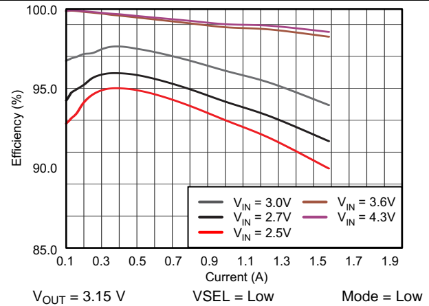
Figure 30. TPS61281A Efficiency vs Output Current
