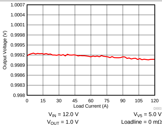
Figure 103. Load Regulation
