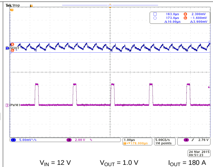
Figure 108. Output Ripple
