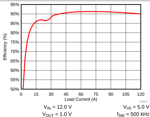
Figure 104. Load Current vs. Efficiency
