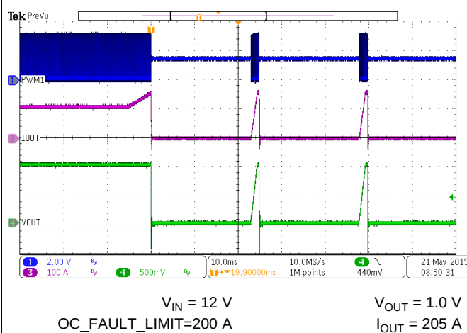
Figure 114. Hiccup mode (OCP)
