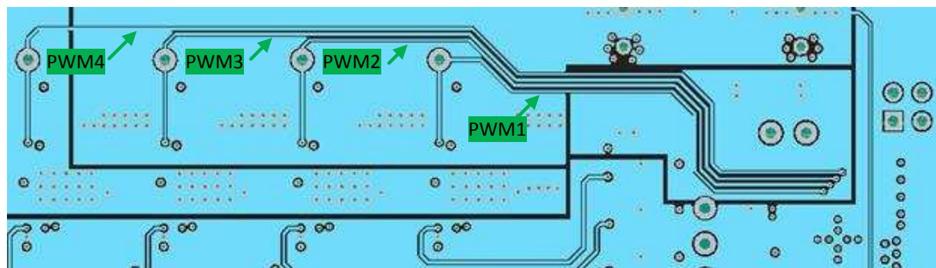
Figure 119. Layout Example for PWM Traces
