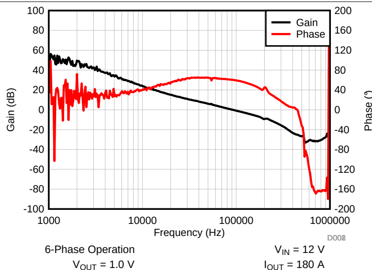
Figure 115. Bode Plot
