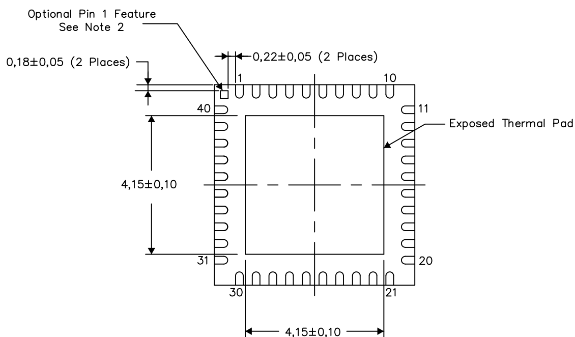
Bottom View
