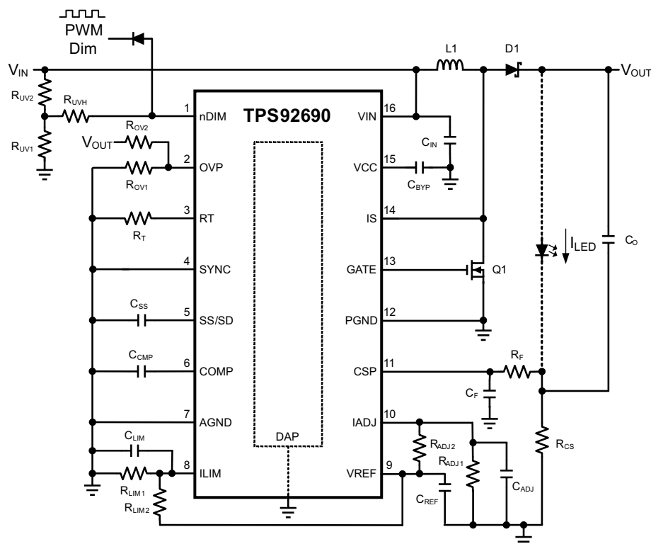
Figure 22. Boost Topology With PWM Dimming
