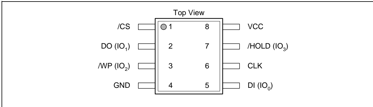
Figure 1a. W25Q80EW Pin Assignments, 8-pin SOIC 150-mil & VSOP 150-mil (Package Code SN, SV)
