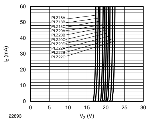
Fig. 8 - Breakdown Characteristics
