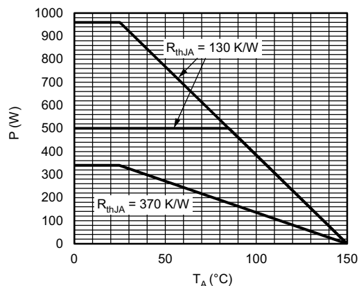
Fig. 3 - Maximum Power Dissipation vs. Ambient Temperature
