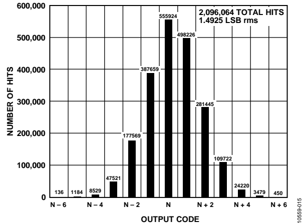
Figure 15. AD9250-170 Grounded Input Histogram
