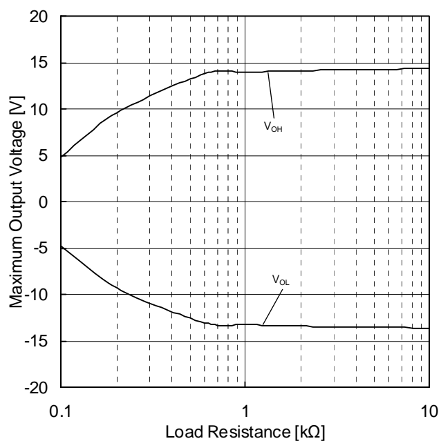
Figure 6. Maximum Output Voltage vs Load Resistance ( V_{CC}/V_{EE}=+15V/-15V , T_A=25^\circ\text{C} )
