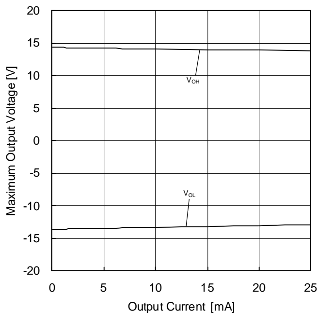
Figure 9. Maximum Output Voltage vs Output Current ( V_{CC}/V_{EE}=+15V/-15V , T_A=25^\circ\text{C} )
