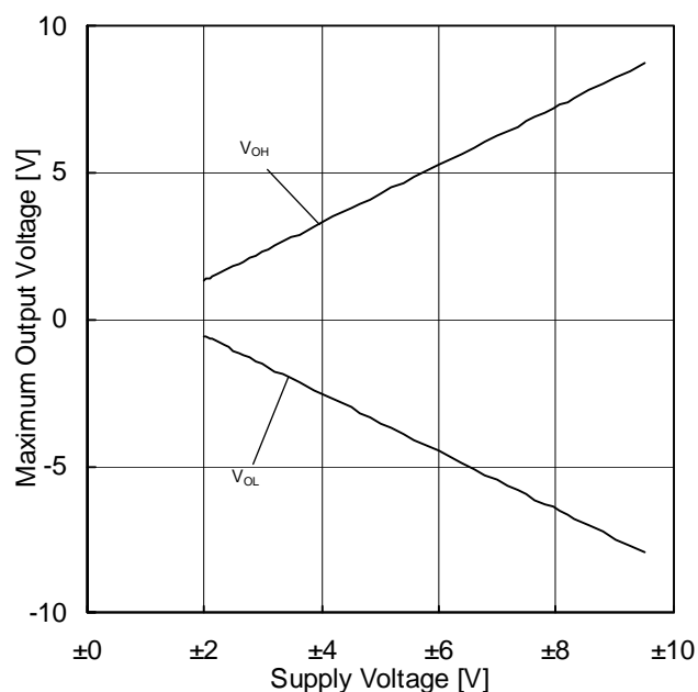
Figure 7. Maximum Output Voltage vs Supply Voltage ( R_L=2k\Omega , T_A=25^\circ\text{C} )
