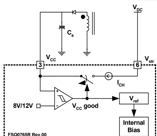
Figure 31. Startup Circuit
