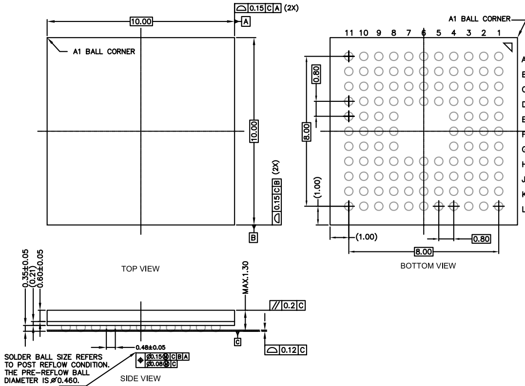
Figure 4.3. BGA112
