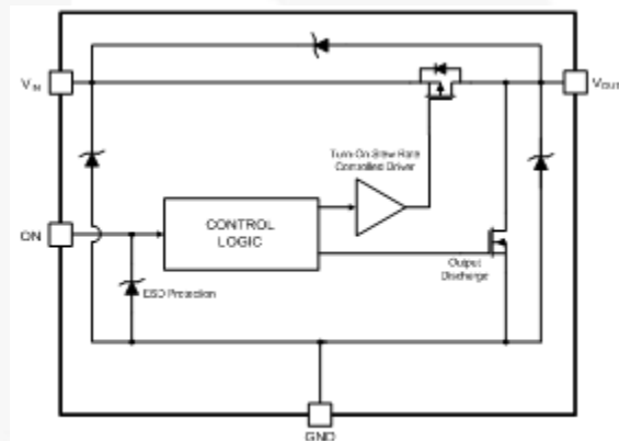
Figure 1. Block Diagram
