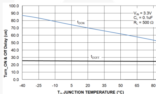
Figure 19. V_{OUT} Turn-On/Turn-Off Delays vs. Temperature ( R_L=500\ \Omega )
