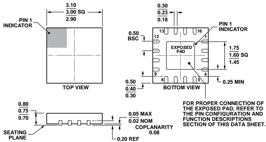
Figure 54. 16-Lead Lead Frame Chip Scale Package [LFCSP_WQ] 3 mm × 3 mm Body, Very Very Thin Quad (CP-16-22) Dimensions shown in millimeters
