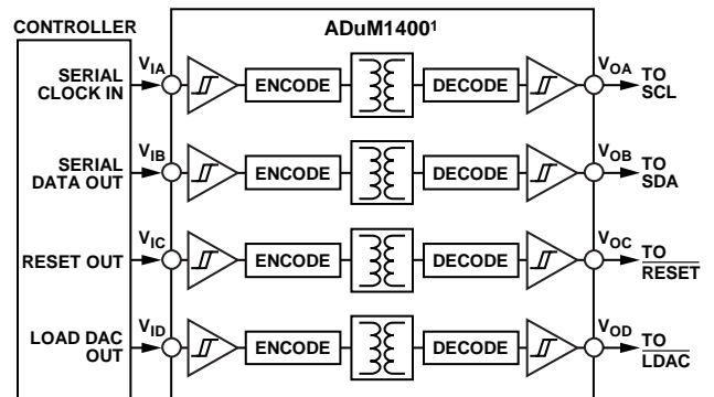
Figure 53. Isolated Interface
