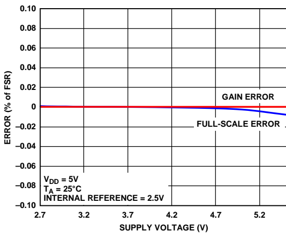
Figure 19. Gain Error and Full-Scale Error vs. Supply Voltage
