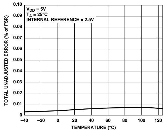
Figure 21. Total Unadjusted Error vs. Temperature
