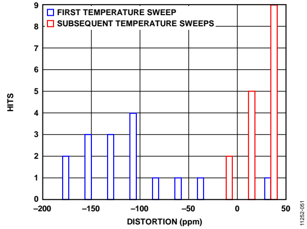
Figure 50. Thermal Hysteresis
