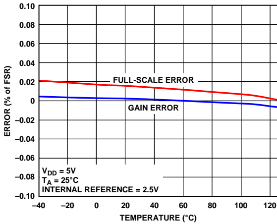
Figure 17. Gain Error and Full-Scale Error vs. Temperature
