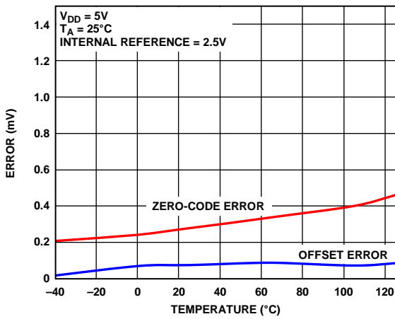
Figure 18. Zero-Code Error and Offset Error vs. Temperature
