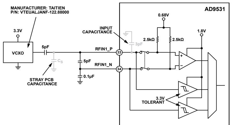
Figure 46. Connecting an External 3.3 V CMOS VCXO Single-Ended Output to the RFIN1_x Pins
