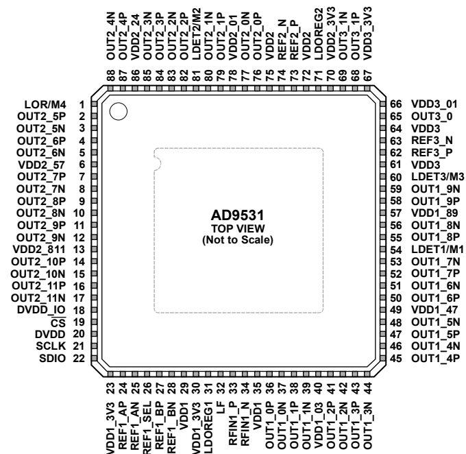
Figure 2. Pin Configuration
