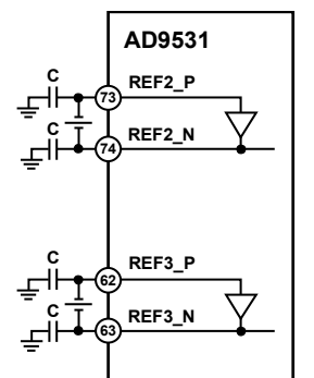
Figure 48. Interfacing the REF2 or REF3 Inputs to a Crystal Resonator
