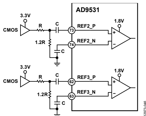
Figure 47. Interfacing the REF2 or REF3 Inputs to 3.3 V CMOS
