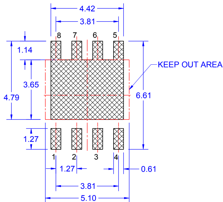
LAND PATTERN RECOMMENDATION
