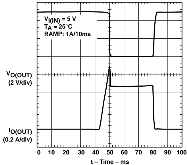
Figure 7. TPS2055A, Threshold Trip Current With Ramped Load on Enabled Device
