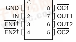
TPS2048A, TPS2058A D PACKAGE (TOP VIEW)
