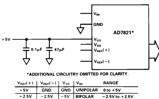
Figure 18. AD7821 Unipolar/Bipolar Operation
