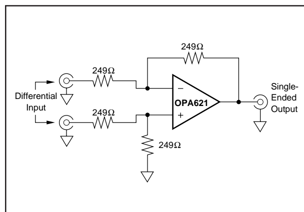
FIGURE 14. Differential Input Buffer Amplifier ( G = -2\text{V/V} ).
