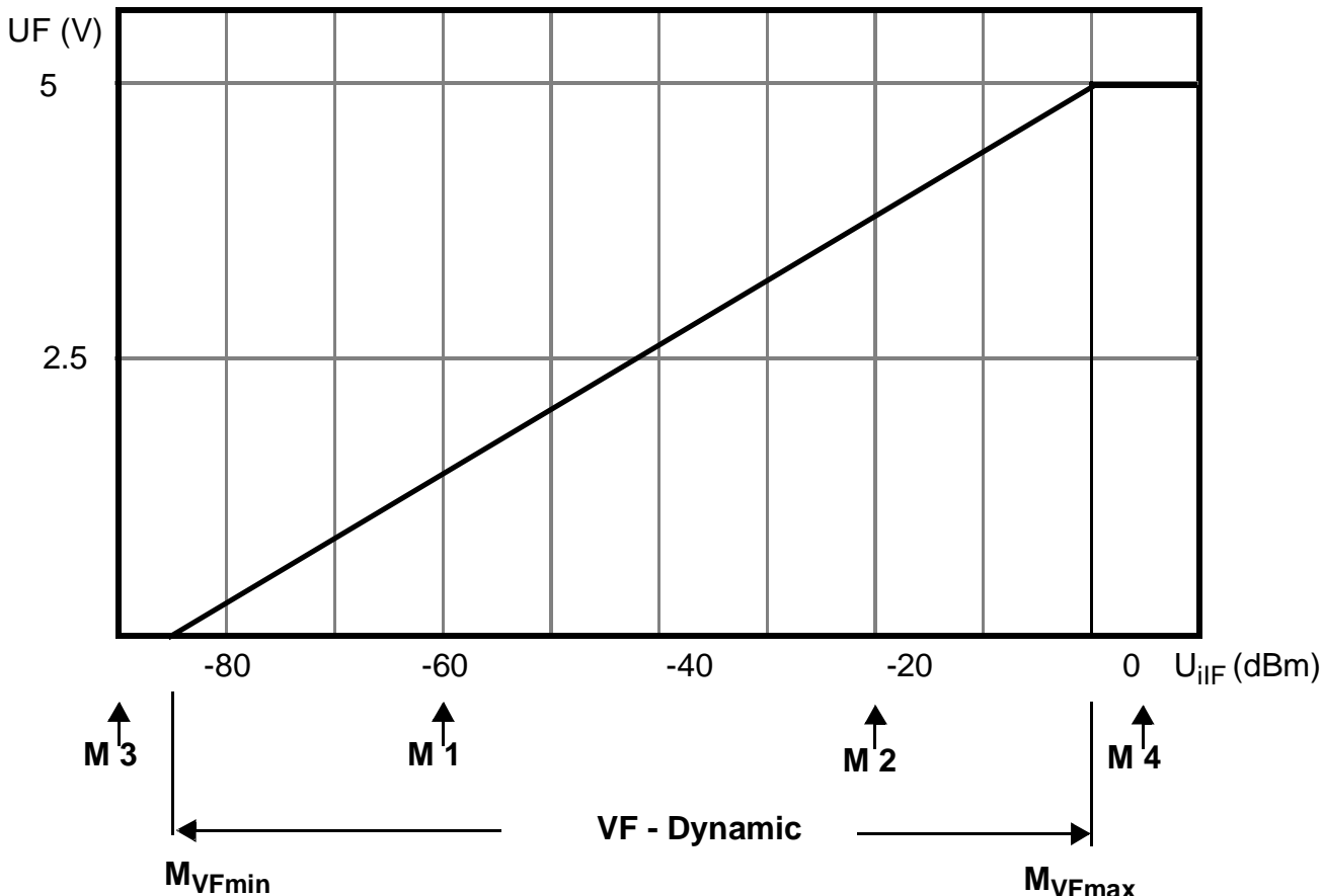
V_F Characteristic
