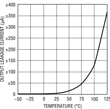
Driver Output Leakage Current (Disable/Shutdown) vs Temperature
