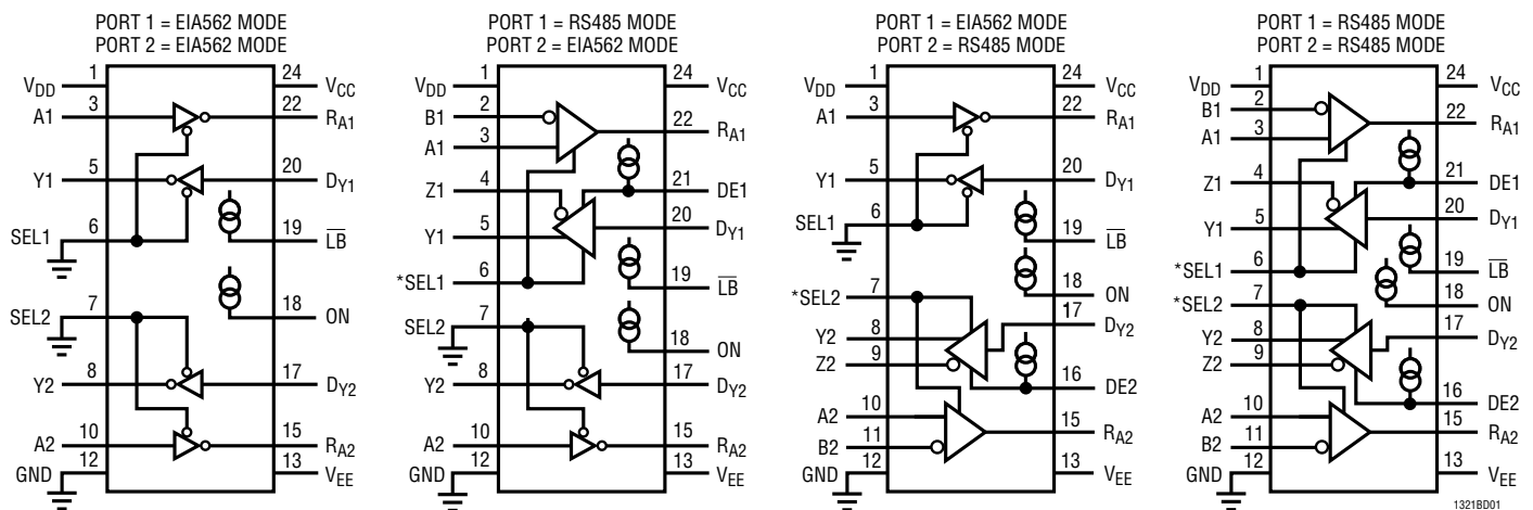
LTC1321 Interface Configuration Without Loopback
