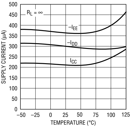
Supply Current in EIA562 Mode vs Temperature (Both Ports)
