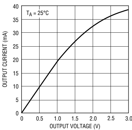
Receiver Output Current vs Output Low Voltage
