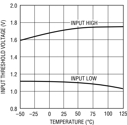
EIA562 Receiver Input Threshold Voltage vs Temperature
