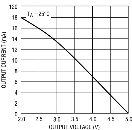
Receiver Output Current vs Output High Voltage
