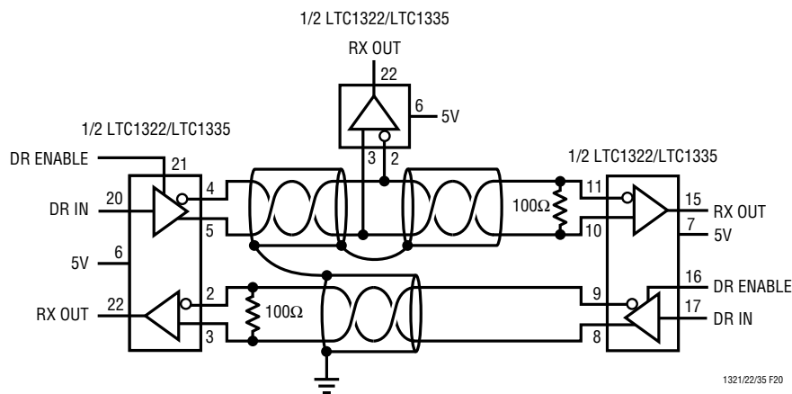
Figure 20. Typical Connection for RS422 Interface
