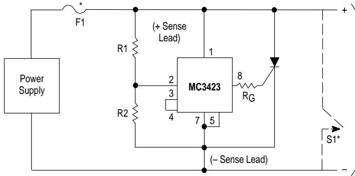
Figure 3. Basic Circuit Configuration
