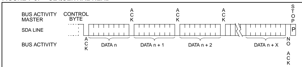
FIGURE 7-3: SEQUENTIAL READ
