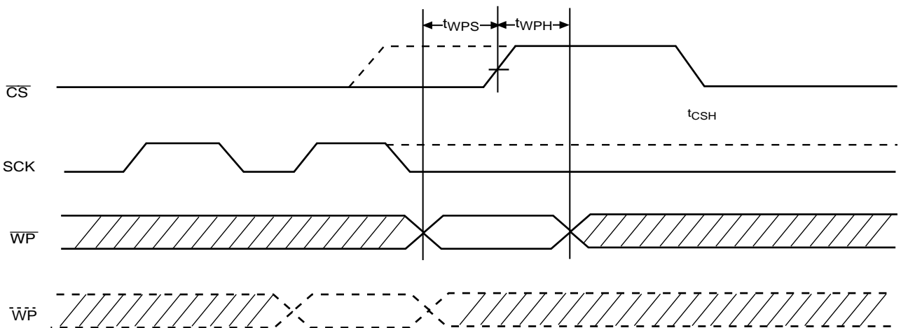
Figure 10. \overline{WP} Timing
