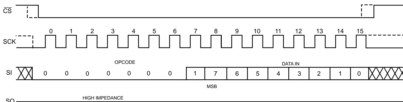
Figure 7. WRSR Timing
