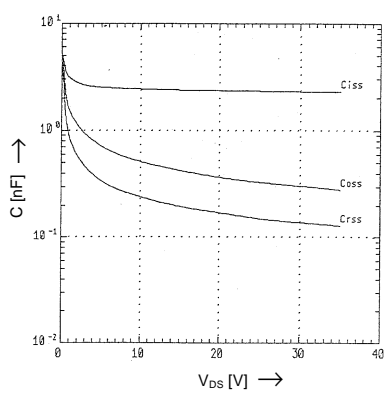
Typical Capacitance vs. V DS
