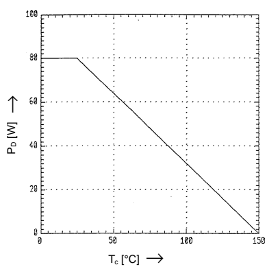
Allowable Power Dissipation vs. T c
