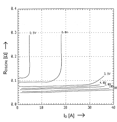
Typical Drain-Source-On-State-Resistance vs. Id
