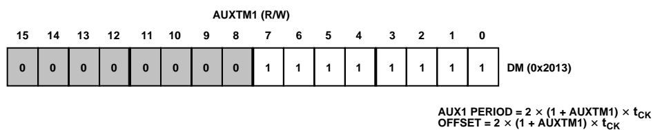
Figure 23. Configuration of AUX Registers
