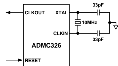
Figure 4. Basic System Configuration
