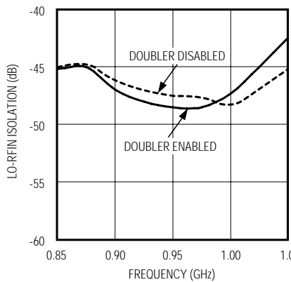
LO-RFIN ISOLATION vs. LO FREQUENCY (INCLUDING BALUN)
