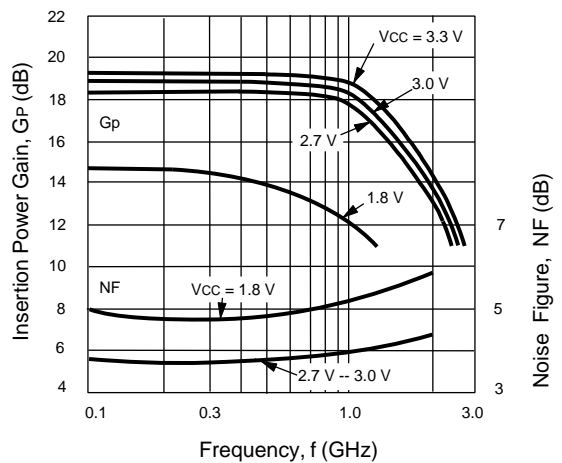
GAIN AND NOISE FIGURE vs. FREQUENCY
