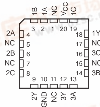
SN54F27 ... FK PACKAGE (TOP VIEW)
