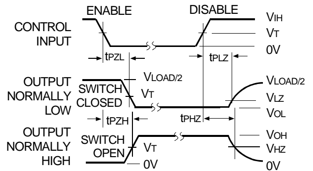
Propagation Delay
