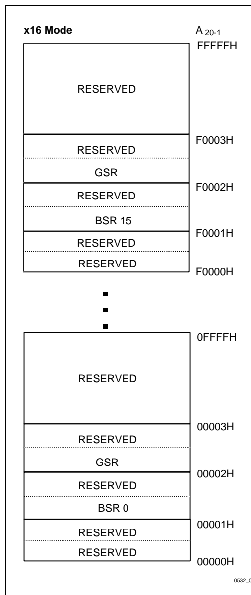
Figure 7. Extended Status Register Memory Map (Word-Wide Mode)
