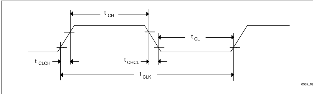
Figure 10. CLK Waveform
