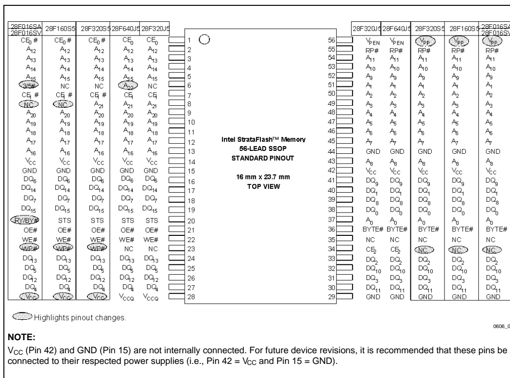
Figure 4. SSOP Lead Configuration (64 Mbit and 32 Mbit)
