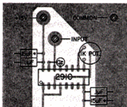
TYPICAL BOARD LAYOUT
