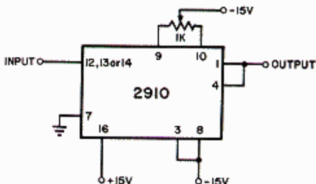
FIGURE 1: BASIC CONNECTIONS
