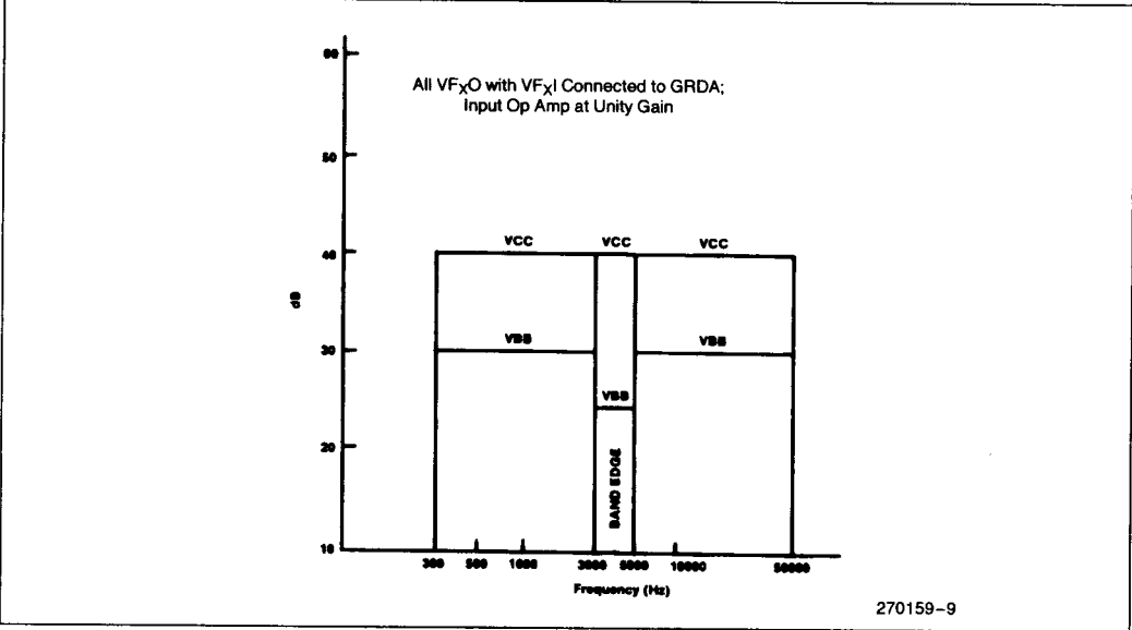
Figure 9. Transmit Filter
