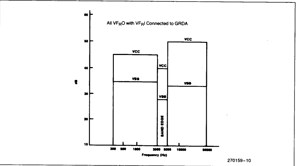
Figure 10. Receive Filter
