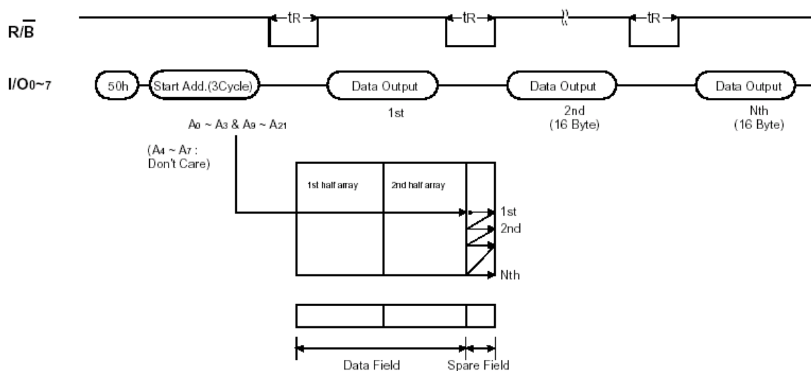
FIGURE 25. SEQUENTIAL READ2 OPERATION ( \overline{SE} = FIXED LOW)
