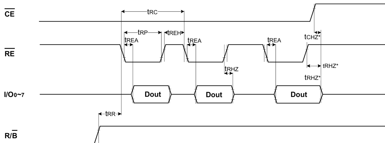
FIGURE 13. SEQUENTIAL OUT CYCLE AFTER READ ( \text{CLE} = \text{L} , \overline{\text{WE}} = \text{H} , \text{ALE} = \text{L} )
