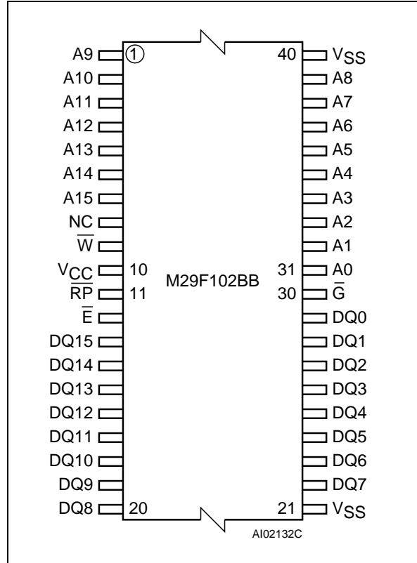
Figure 4. TSOP Connections
