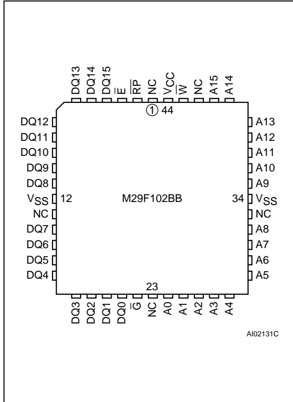
Figure 3. PLCC Connections
