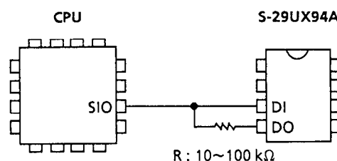
Figure 8 3-wire interface
