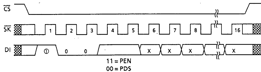
Figure 7 PEN/PDS Timing
