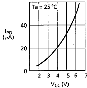
1.9 Pull-Down current I_{PD} — Power supply voltage V_{CC}
