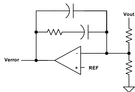
FIGURE 11. TYPE 2 ERROR AMPLIFIER
