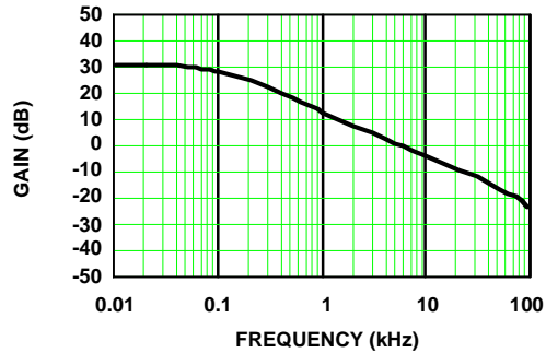
FIGURE 12A. GAIN
