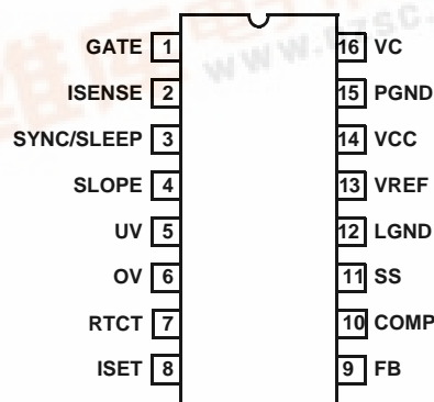
ISL6722A, ISL6723A (SOIC, TSSOP) TOP VIEW
