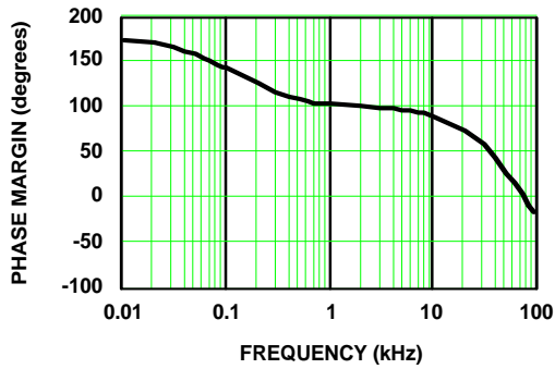
FIGURE 12B. PHASE MARGIN
