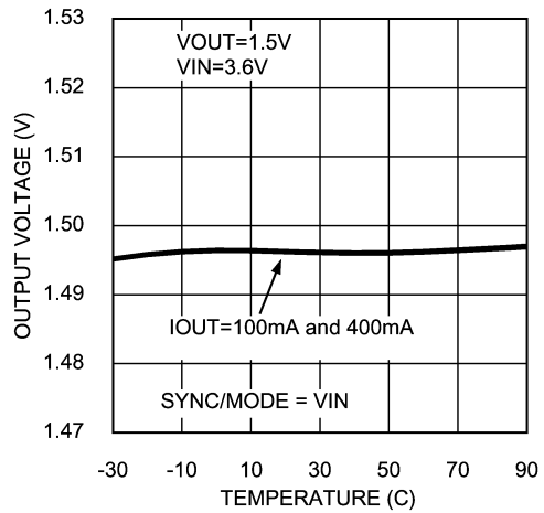
Output Voltage vs Temperature (PWM Mode)
