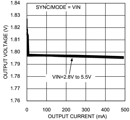
Output Voltage vs Output Current ( V_{OUT} = 1.8V , PWM Mode)
