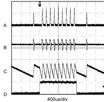
Load Transient Response (PFM Mode)
