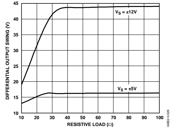
Figure 26. Differential Output Swing vs. R_{LOAD} ADSL/ADSL2+ Circuit (Figure 32)
