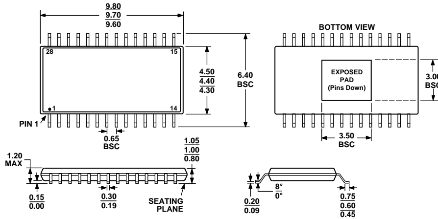
Figure 41. 28-Lead Thin Shrink Small Outline with Exposed Pad [TSSOP/EP]
