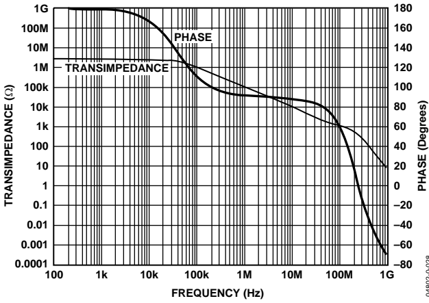
Figure 28. Open-Loop Transimpedance and Phase
