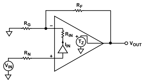
Figure 33. Simplified Block Diagram
