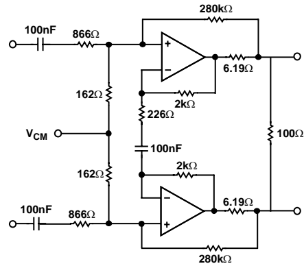
Figure 32. ADSL/ADSL2+ Circuit
