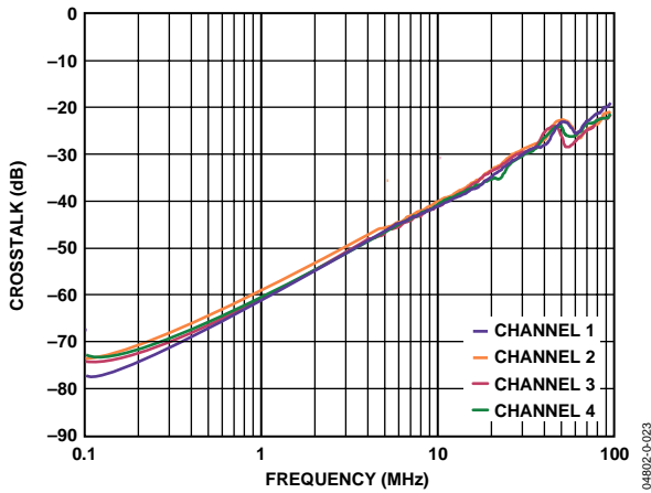
Figure 23. Crosstalk vs. Frequency Quad Op Amp Circuit (Figure 29)
