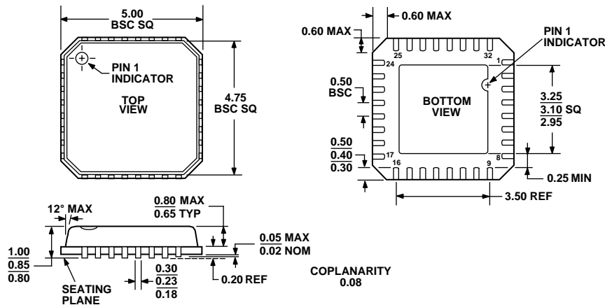
Figure 42. 32-Lead Lead Frame Chip Scale Package [LFCSP]
