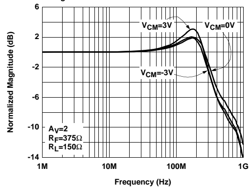
Frequency Response for Various Common-Mode Input Voltages
