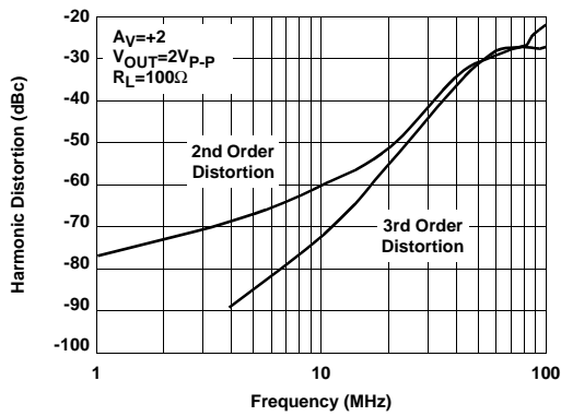
2nd and 3rd Harmonic Distortion vs Frequency
