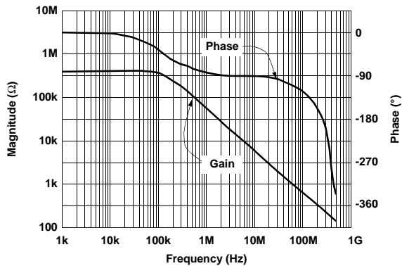
Transimpedance (ROL) vs Frequency
