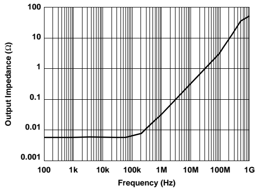
Closed Loop Output Impedance vs Frequency
