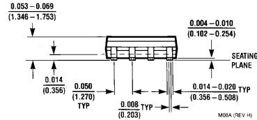
8-Lead (0.150") Molded Small Outline Package, JEDEC Ordering Number LM6152ACM or LM7162BCM NSC Package Number M08A
