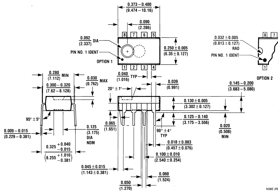
8-Lead (0.300" Wide) Molded Dual-In-Line Package, JEDEC Order Number LM615ACN or LM6152BCN NSC Package Number N08E
