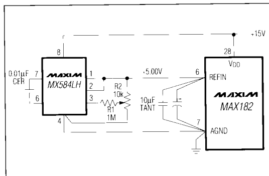
Figure 19. MX584LH as Reference Generator
