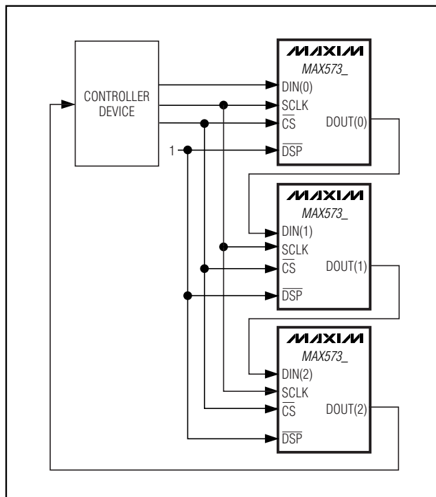
Figure 4. Daisy-Chain Configuration
