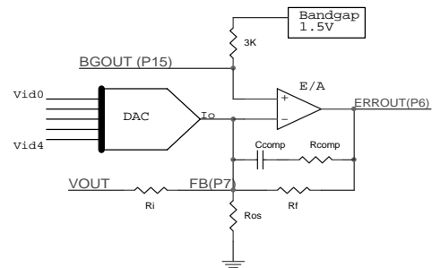
Figure 2: Error amplifier connections
