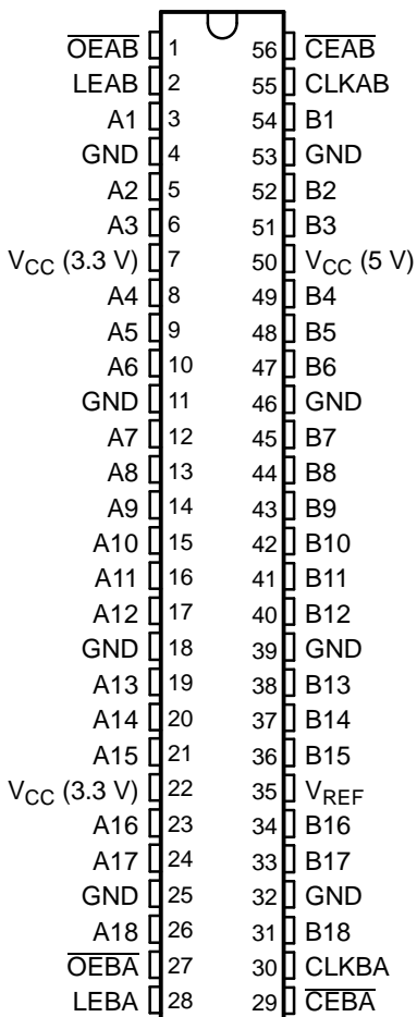
SN54GTL16612A... WD PACKAGE SN74GTL16612A... DGG OR DL PACKAGE (TOP VIEW)
