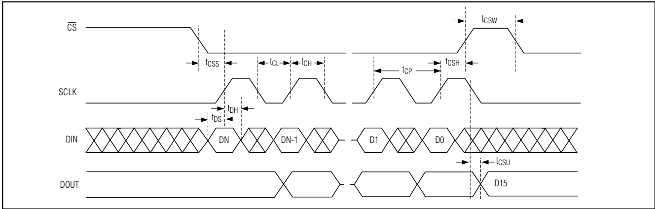
Figure 6. 4-Wire Serial Interface Timing Diagram
