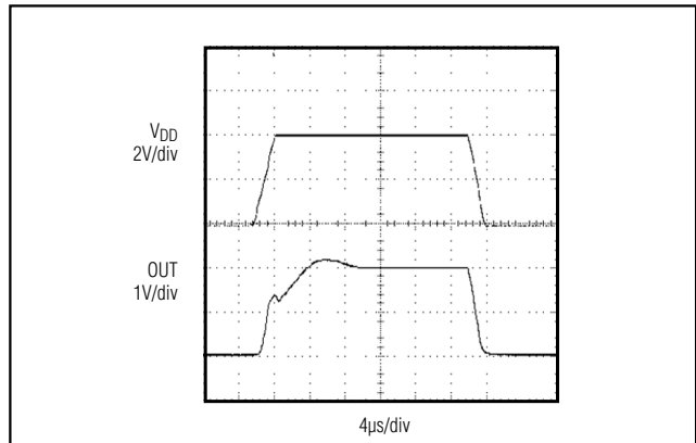
Figure 5. Power-Up/Down Waveform
