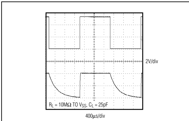
Figure 4. Shutdown Waveform
