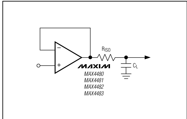
Figure 3. Capacitive-Load-Driving Circuit
