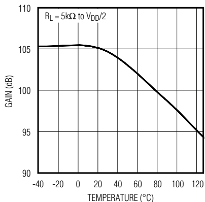
LARGE-SIGNAL GAIN vs. TEMPERATURE
